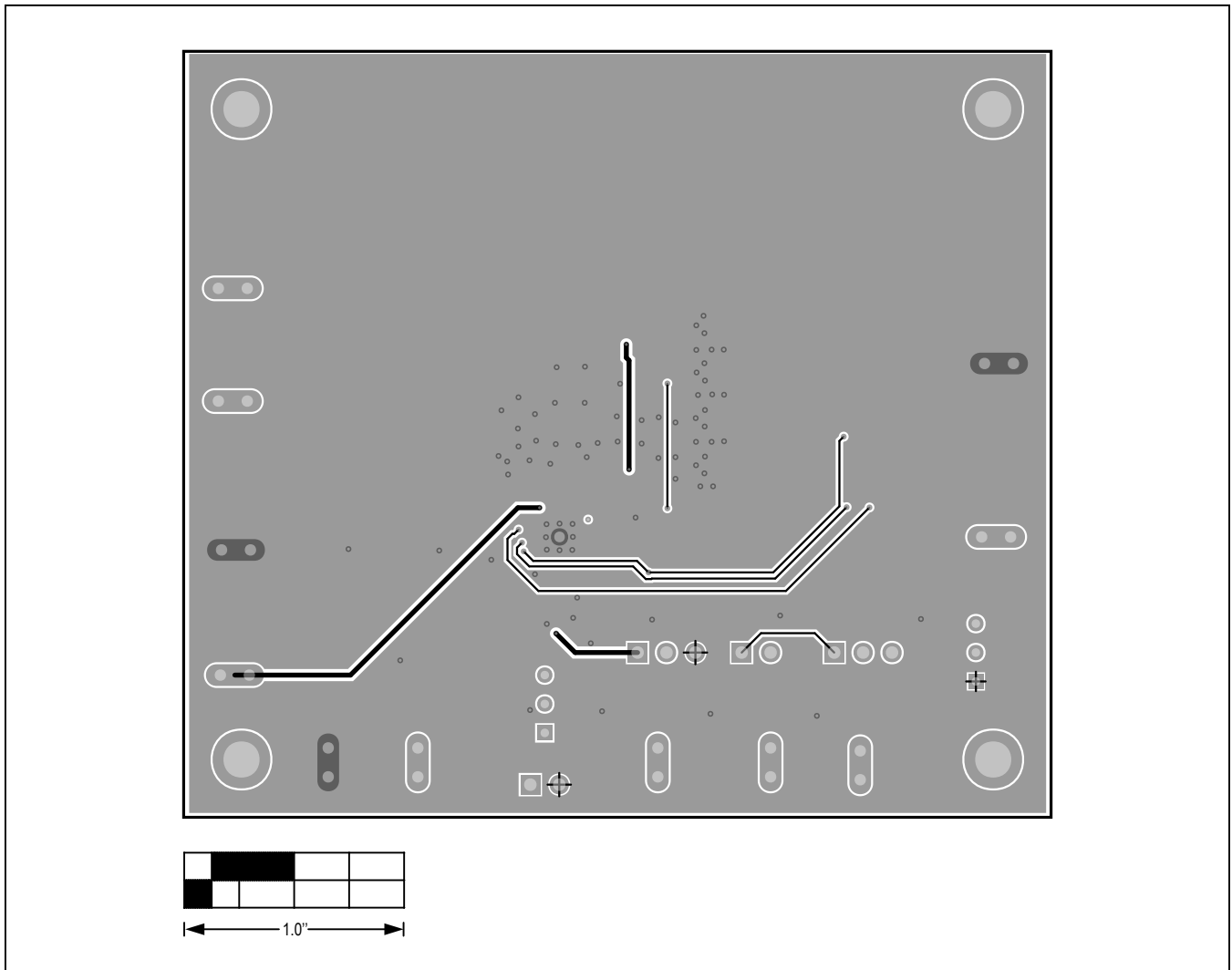
PCB Layout—Bottom
