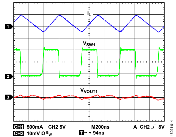
Figure 25. SW1 Waveform, V_{VOUT1} = 5V , I_{VOUT1} = 100mA
