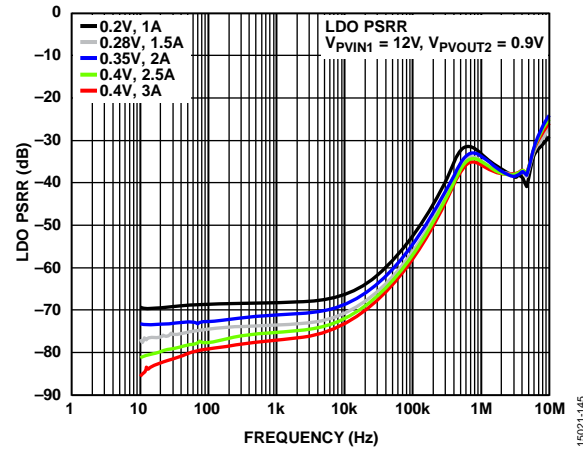
Figure 49. LDO PSRR vs. Frequency
