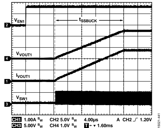
Figure 36. Buck Startup
