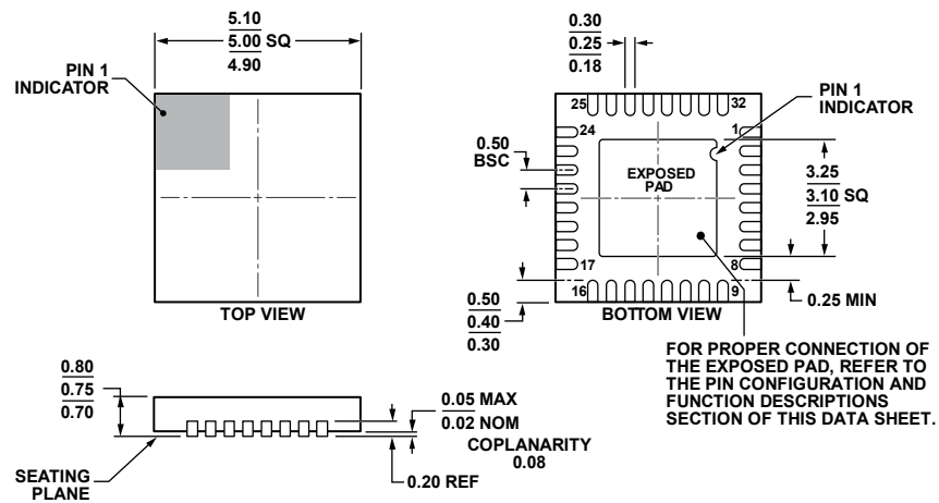
COMPLIANT TO JEDEC STANDARDS MO-220-WHHD. Figure 52. 32-Lead Lead Frame Chip Scale Package [LFCSP] 5 mm × 5 mm Body and 0.75 mm Package Height (CP-32-7) Dimensions shown in millimeters
