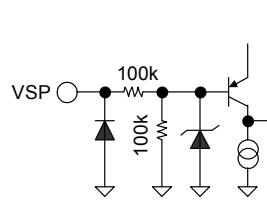
Figure 49. VSP
