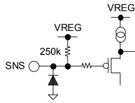
Figure 48. SNS
