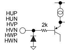
Figure 52. HXP, HXN
