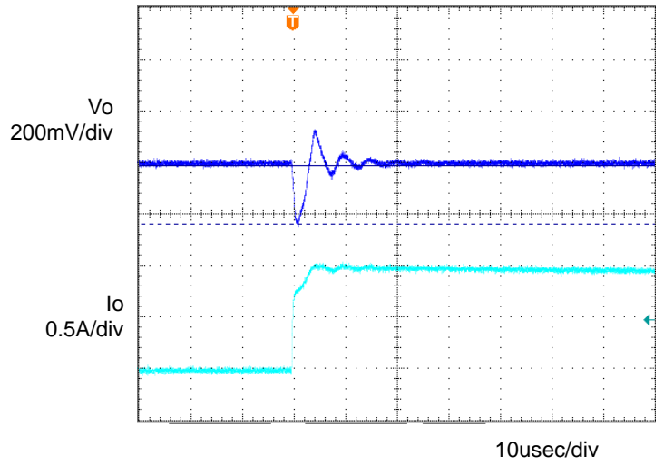
Figure 4. Transient Response (1.0→0A) Co=1μF, Ta=25°C
