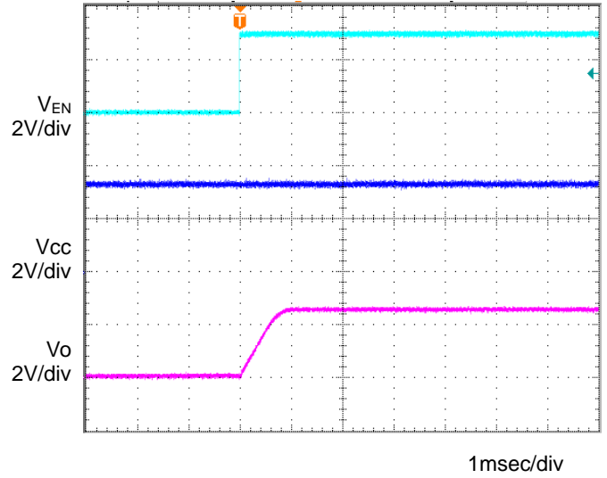
Figure 16. Input sequence 2 Co=1μF, Ta=25°C
