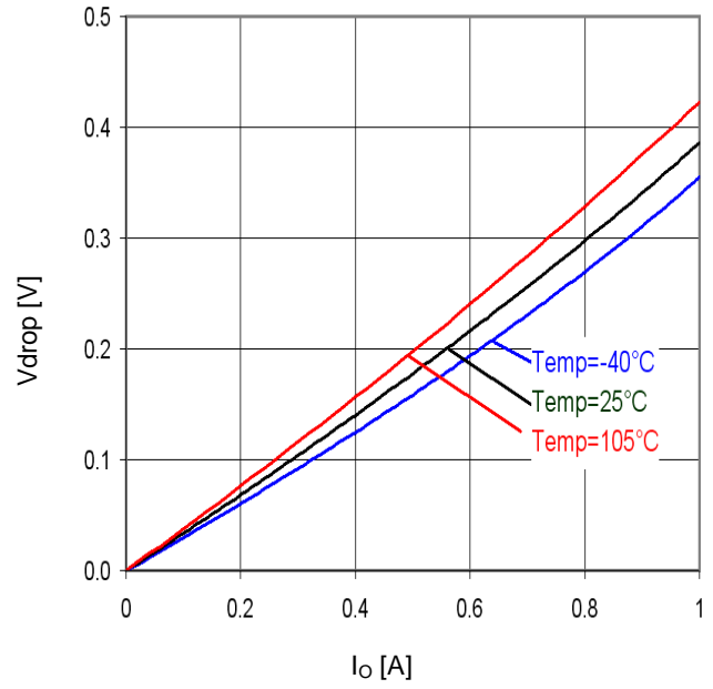
Figure 36. Minimum dropout Voltage 2 (VCC=4V, Ta=25°C)
