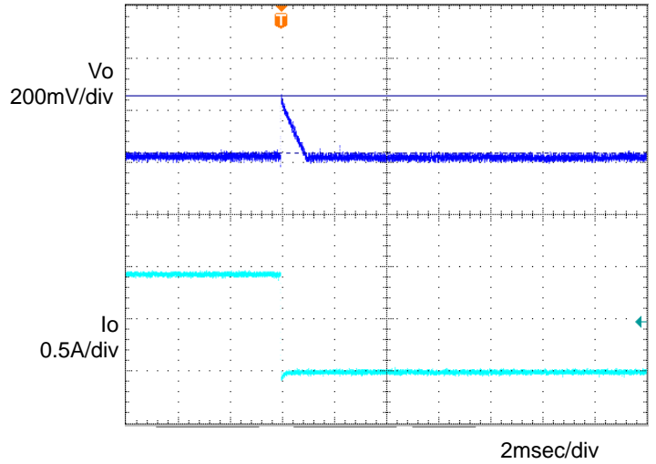
Figure 6. Transient Response (1.0→0A) Co=1μF, Ta=-40°C
