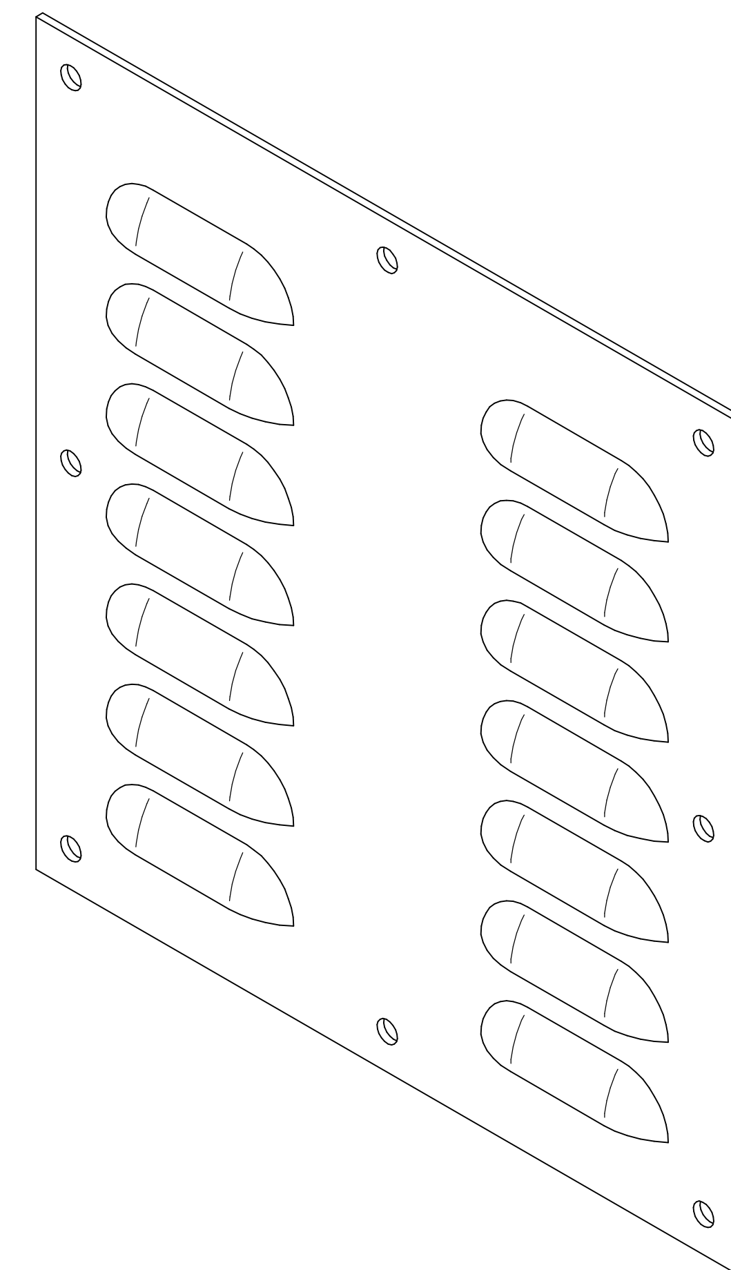
ISOMETRIC VIEW
