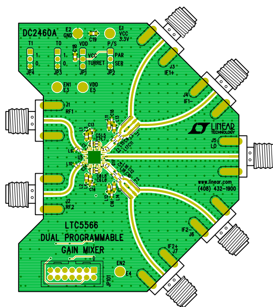
Figure 1. DC2460A
