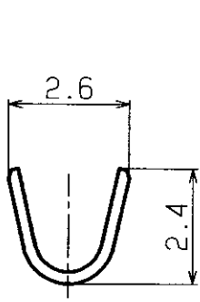
WIRE BARREL
