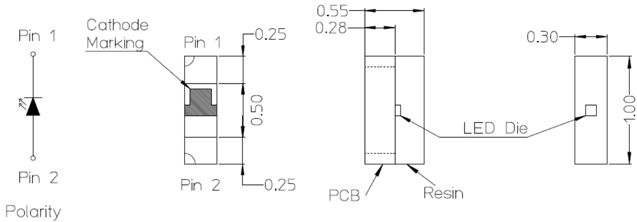
Figure 1: Package Dimensions
