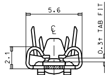
VIEW "A"
