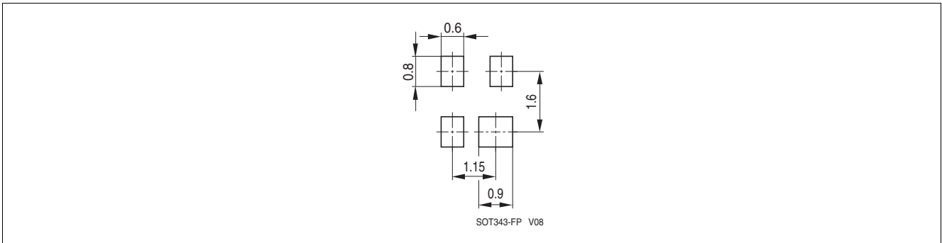
Figure 23 Package Foot Print
