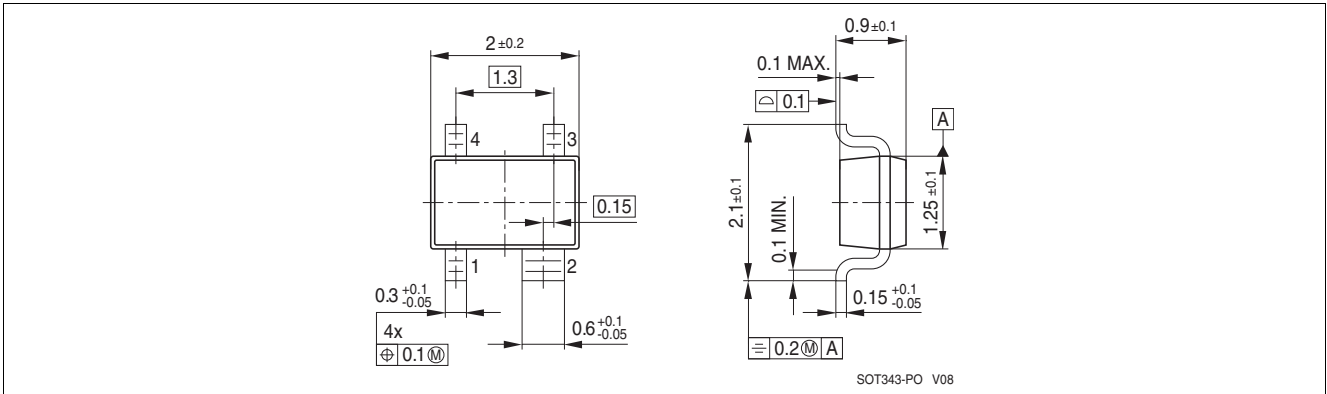
Figure 22 Package Outline
