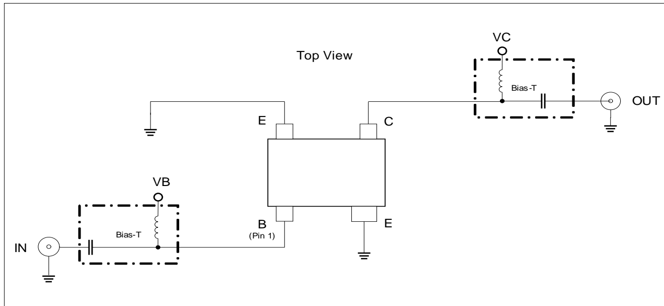
Figure 2 BFP840ESD Testing Circuit
