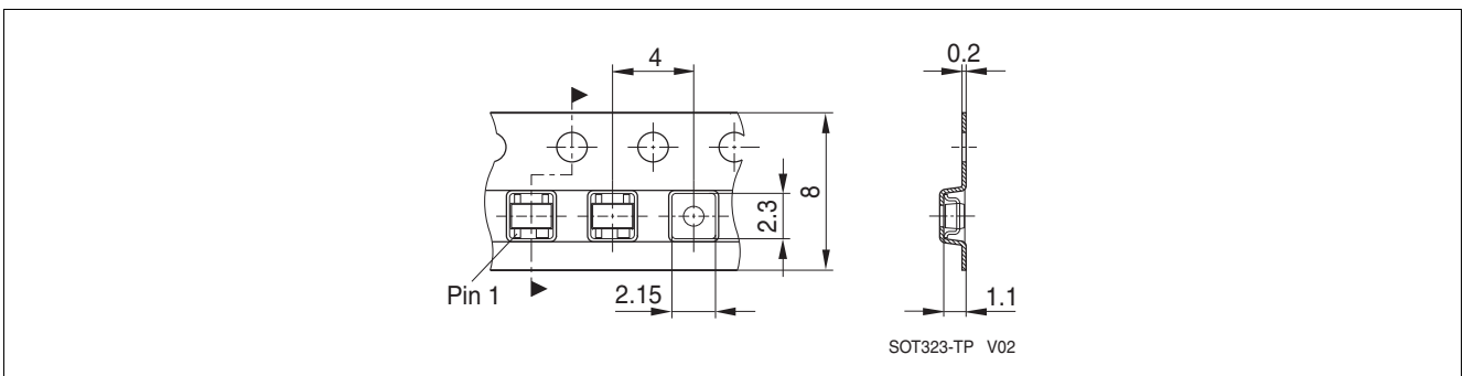
Figure 25 Tape Dimensions
