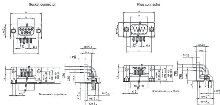
Socket connector:
