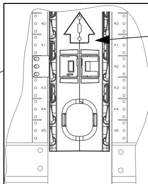
Rear Bottom Mounting Location
