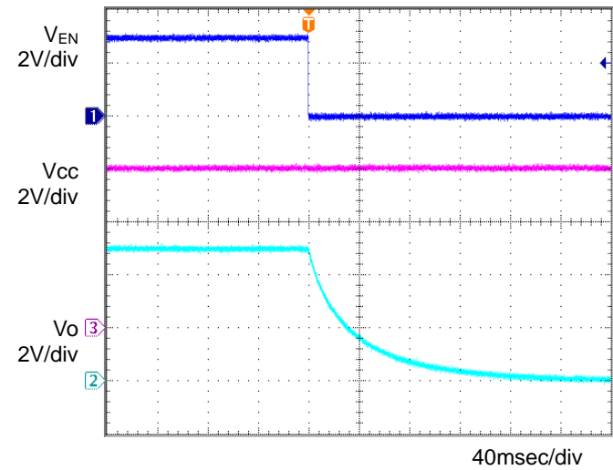
Figure 18. OFF sequence 2 Co=1μF, Ta=-40°C
