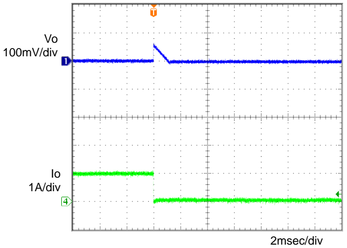
Figure 6. Transient Response (1.0→0A) Co=1µF, Ta=-40°C
