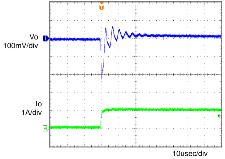
Figure 4. Transient Response (0→1.0A) Co=1µF, Ta=25°C
