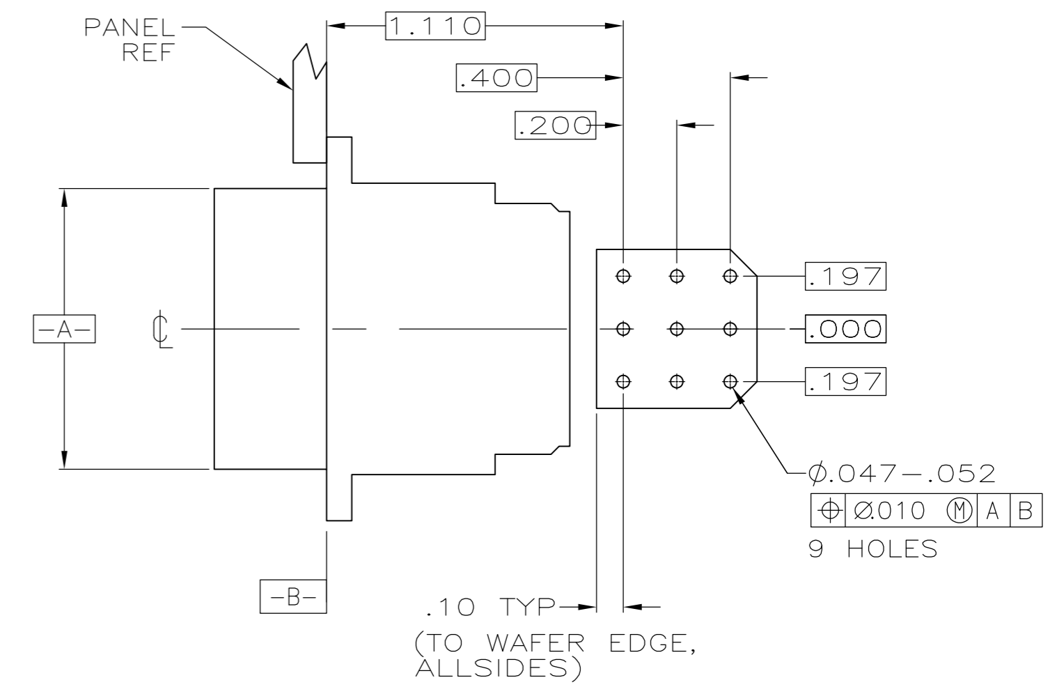
VIEW A-A \triangle RECOMMENDED PC BOARD LAYOUT
