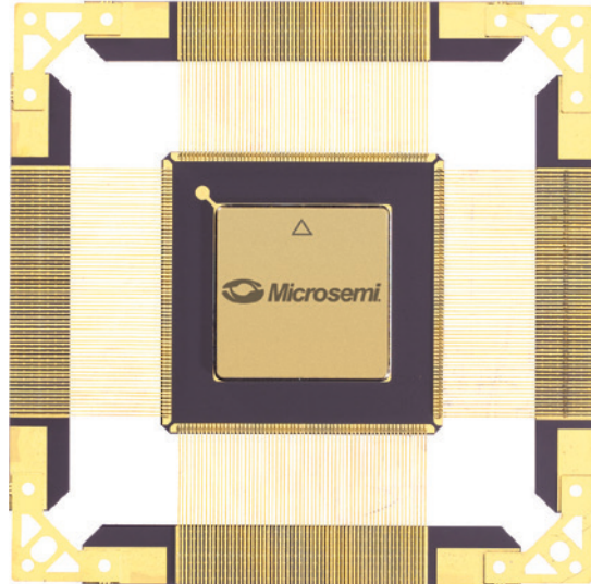
CQ256 b.s. 1.417" x 1.417" (36 mm x 36 mm) h. 105 mils (2.67 mm) p. 20 mils (0.50 mm)
