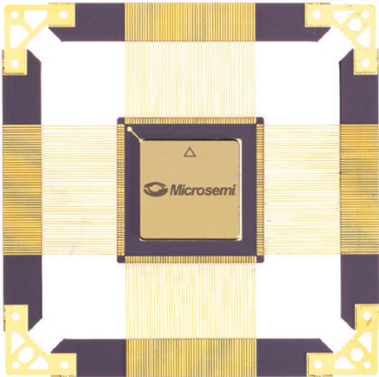
CQ208 b.s. 1.15" x 1.15" (29.21 mm x 29.21 mm) h. 105 mils (2.67 mm) p. 20 mils (0.50 mm)
