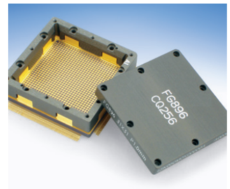
RTAX2000S CQ256 to FG896 Ceramic Adapter, Top & Bottom
