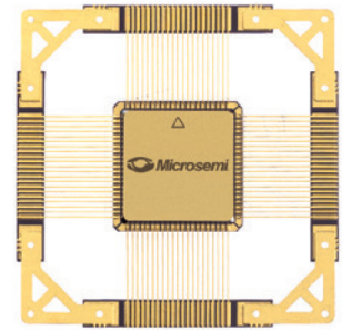
CQ84 b.s. 0.65" x 0.65" (16.51 mm x 16.51 mm) h. 90 mils (2.29 mm) p. 25 mils (0.64 mm)
