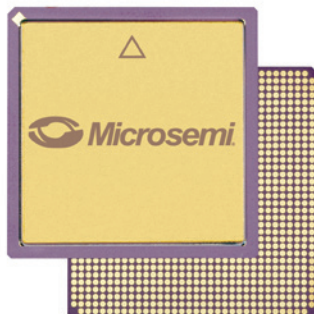
CG1152/LG1152 RTAX2000S & RTAX2000SL only b.s. 1.378" x 1.378" (35 mm x 35 mm) h. CCGA—218 mils (5.535 mm) h. LGA—129 mils (3.28 mm) p. 39 mils (1.00 mm)
