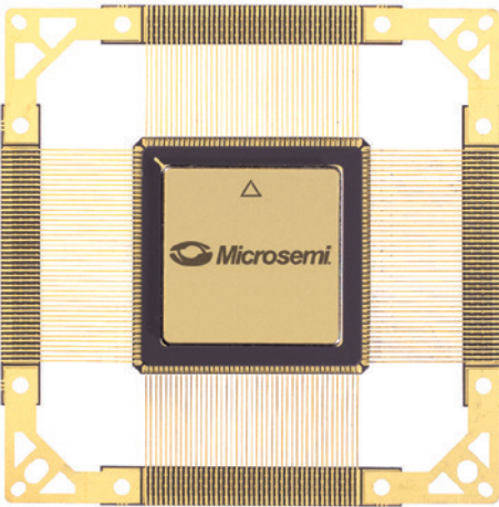
CQ172 b.s. 1.18" x 1.18" (29.972 mm x 29.972 mm) h. 105 mils (2.67 mm) p. 25 mils (0.64 mm)
