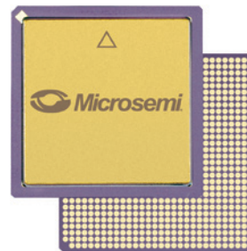
CG896/LG896 b.s. 1.220" x 1.220" (31 mm x 31 mm) h. CCGA—218 mils (5.535 mm) h. LGA—129 mils (3.28 mm) p. 39 mils (1.00 mm)
