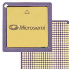
b.s. 0.91" x 0.91" (23.00 mm x 23.00 mm) h. CCGA—225 mils (5.72 mm) h. LGA—138 mils (3.51 mm) p. 7.5 mils (0.19 mm)
