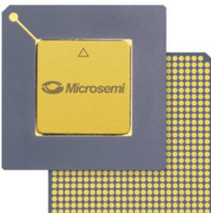
b.s. 1.27" x 1.27" (32.50 mm x 32.50 mm) h. CCGA—194 mils (4.94 mm) h. LGA—90 mils (2.30 mm) p. 50 mils (1.27 mm)
