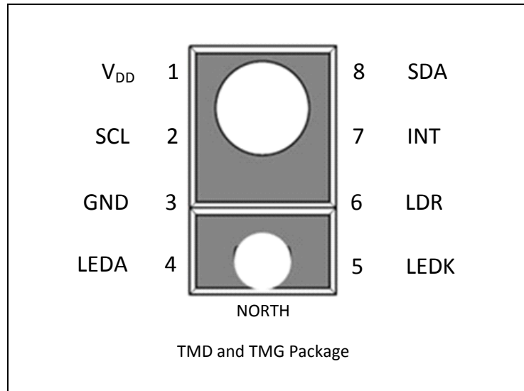
Figure 3: Pin Diagram
