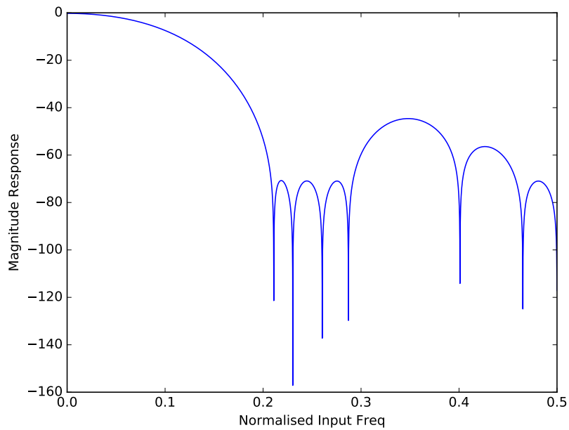
Figure 14: Second stage FIR magnitude response.
