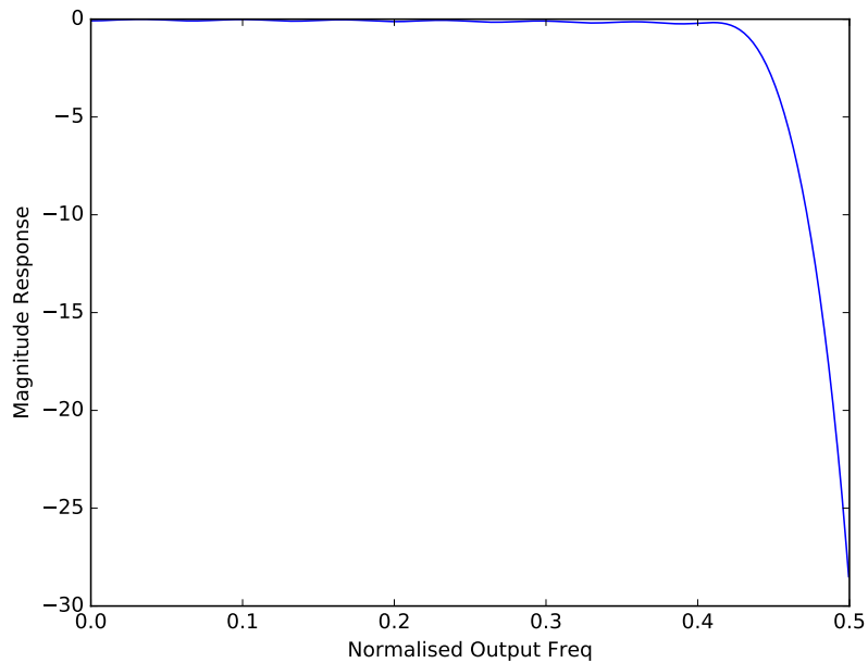
Figure 22: Final frequency response for a divide of 6 giving a typical output rate of 16kHz(3.072MHz) or 14.7kHz(2.8224MHz).
