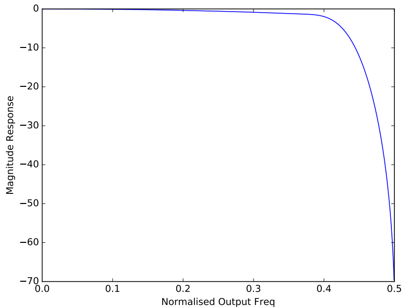
Figure 20: Final frequency response for a divide of 2 giving a typical output rate of 48kHz(3.072MHz) or 44.1kHz(2.8224MHz).
