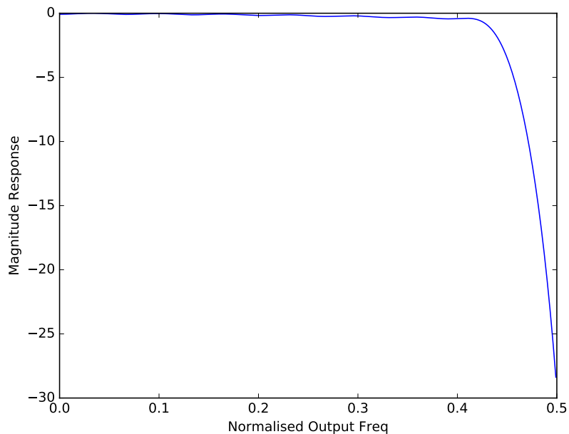
Figure 21: Final frequency response for a divide of 4 giving a typical output rate of 24kHz(3.072MHz) or 22.05kHz(2.8224MHz).
