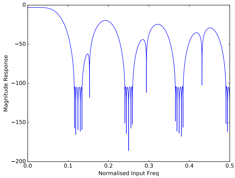
Figure 13: First stage FIR magnitude response.
