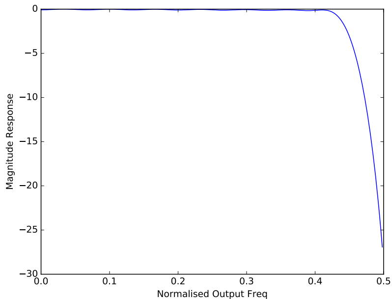
Figure 23: Final frequency response for a divide of 8 giving a typical output rate of 12kHz(3.072MHz) or 11.025kHz(2.8224MHz).
