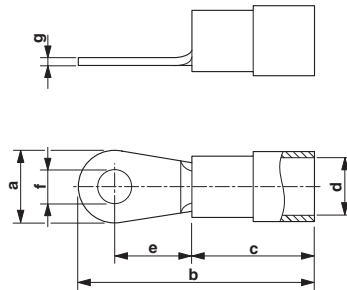
Dimensioned drawing
