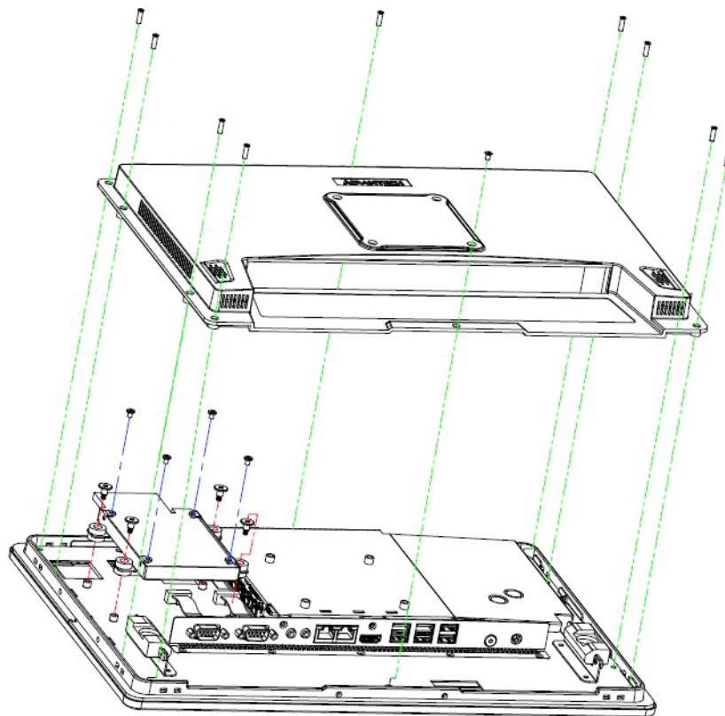
Figure 3.1 Installing primary 2.5" HDD
