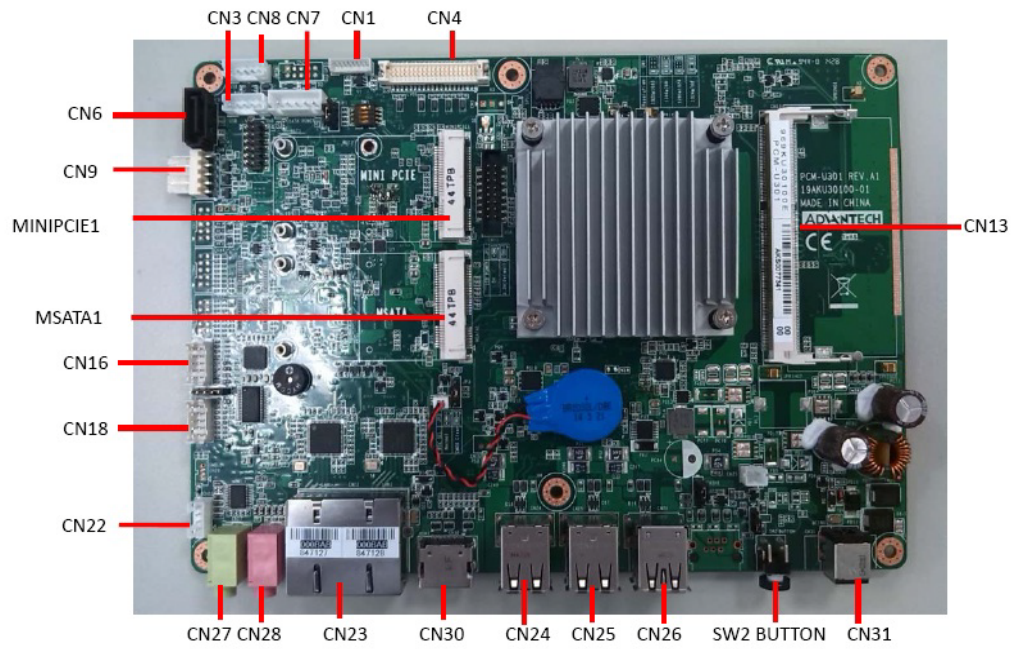
Figure 4.1 Jumpers and Connectors on the UTC-315 motherboard
