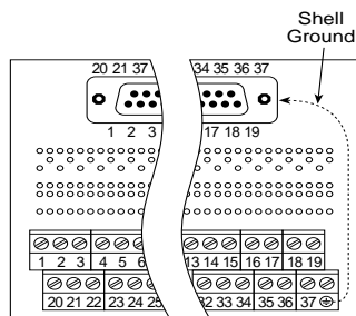
Female Connector SD-F37 37 Pin Socket Female Connector Shown with component mounting holes (pads are on solder side)
