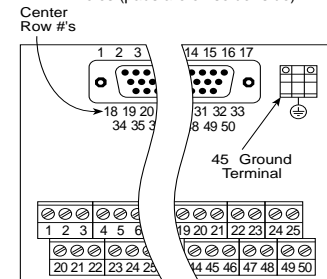
Male Connector SD-M50 50 Pin Male Connector Shown with no component solder pads
