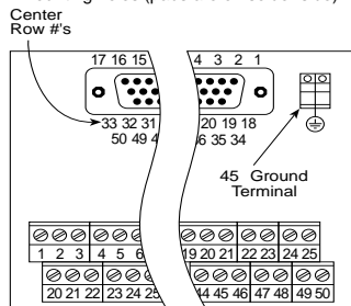
Female Connector SD-F50 50 Pin Socket Female Connector Shown with no component solder pads
