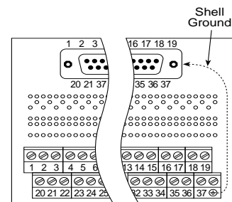
Male Connector SD-M37 37 Pin Male Connector Shown with component mounting holes (pads are on solder side)
