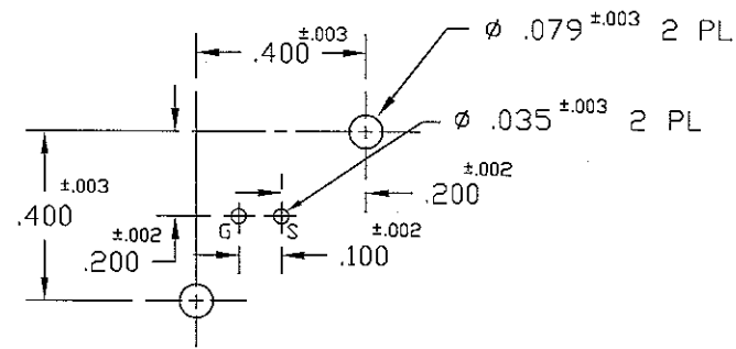
PC HOLE MOUNTING
