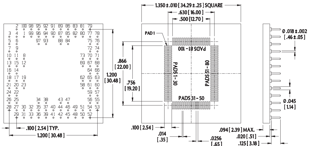
X-RAY VIEW TOP SIDE QFP PAD ASSIGNMENT
