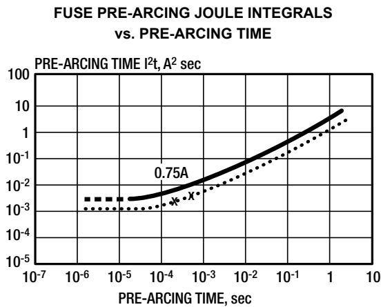
Fig.5b. Choice of fuse, example #5 — Pre-arcing I 2 t - - - - - Maximum I 2 t design rule x I 2 t for sample switch-on pulse
