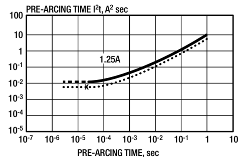
Fig. 4c. Choice of 0.5A fuse, example #4. — Pre-arcing I^2t - - - Maximum I^2t design rule x I^2t for sample current pulse
