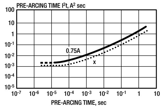
Fig. 6b. Choice of 0.75A fuse, example #6. — Pre-arcing I 2 t - - - - - Maximum I 2 t design rule x I 2 t for sample current pulse
