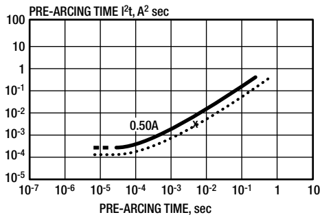
Fig. 3c. Choice of 0.75A fuse, example #3. — Pre-arcing I^2t - - - Maximum I^2t design rule x I^2t for sample current pulse
