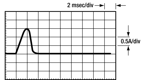
Fig. 2b. Triangular pulse, example #2.
