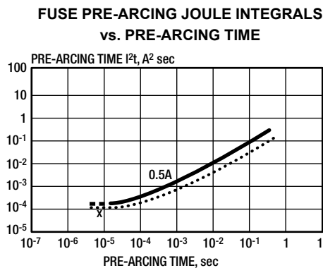
Fig. 1c. Choice of 0.5A fuse, example #1.
