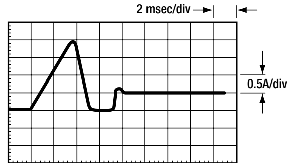
Fig. 6a. Switch-on pulse and steady-state current, example #6
