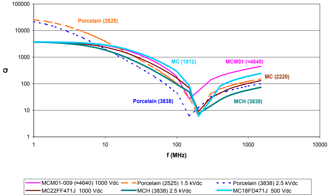
Q vs. Frequency 470 pF @ 25 °C
