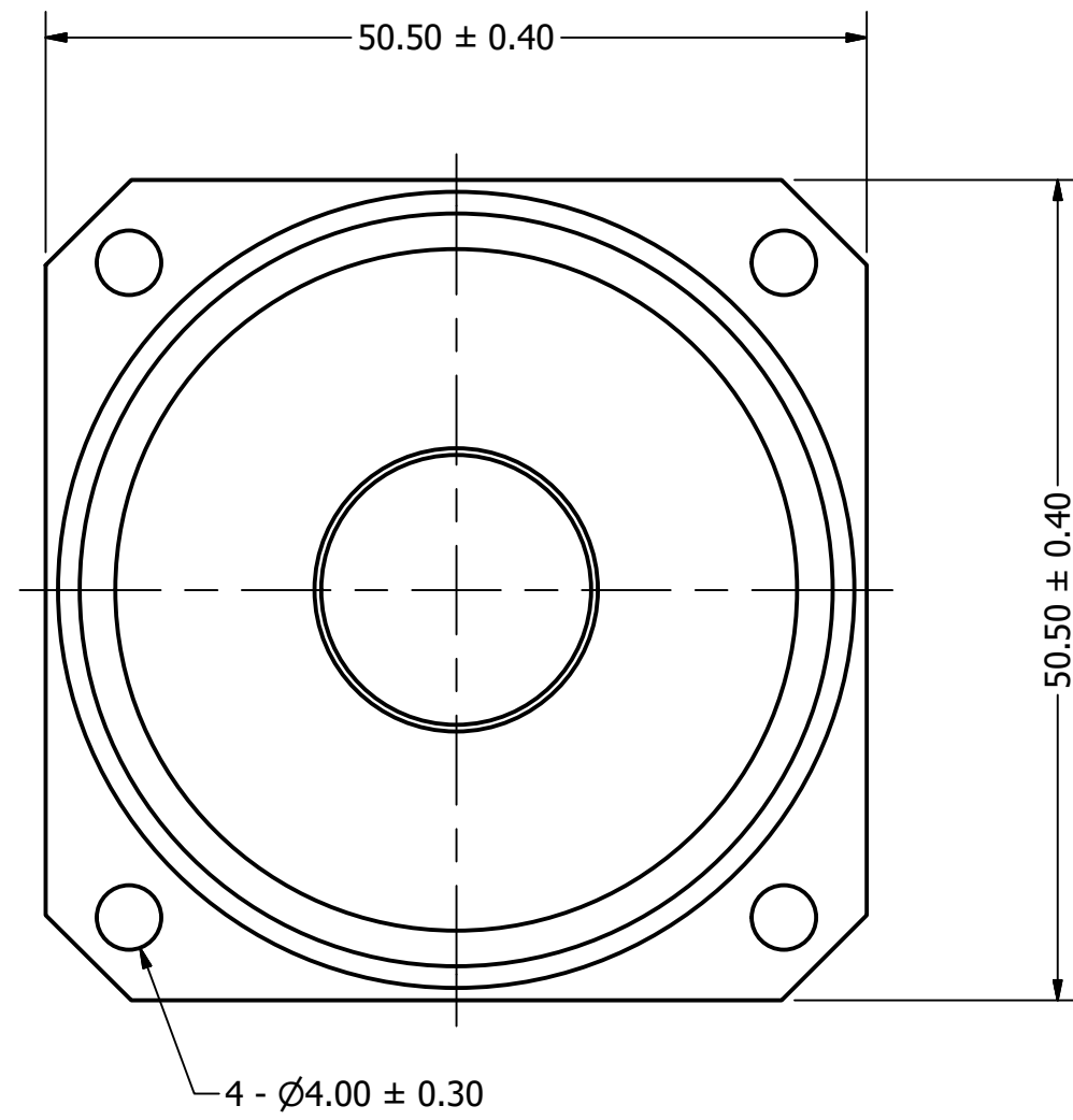
Top View
