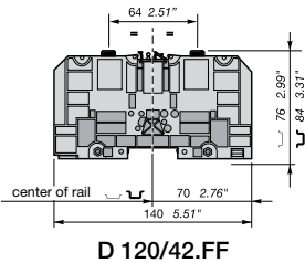
D 120/42.FF
