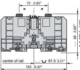
D 300/55.FF
