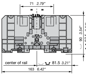
D 185/55.FF
