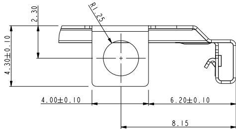
DETAIL B SCALE 4.000
