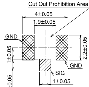
Recommended PCB mounting pattern
