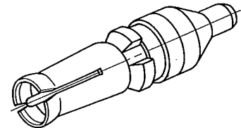
Receptacle type contact (with center contact being male and outer female)
