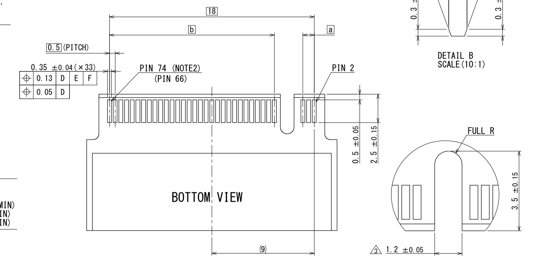
APPLICABLE MODULE DIMENSION (REF.) SCALE (5:1)
