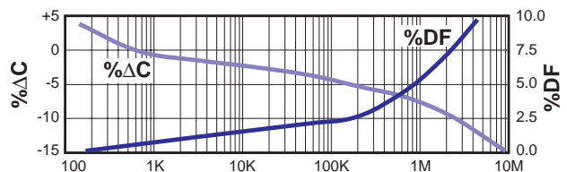
Figure 9. Frequency - Hertz Capacitance & DF vs Frequency - X7R & Z5U
