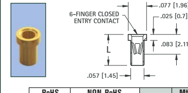
.025 (.64) - .037 (.94) PIN - SOLDER MOUNT
