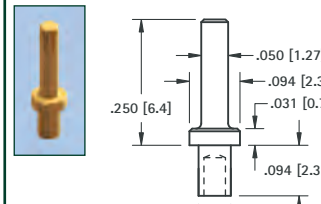
.050 (1.3) PIN - SWAGE MOUNT
