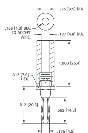
.175 (4.5) Plug
