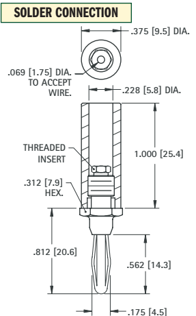
.175 (4.5) Plug
