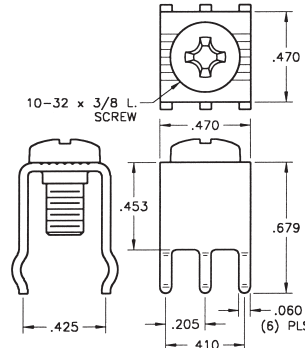
Mounting Detail
