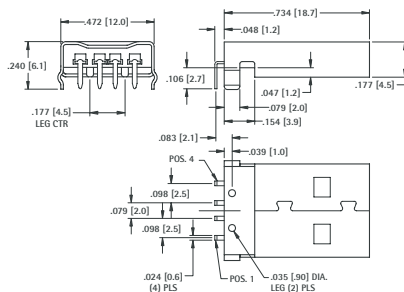
Mounting Detail
