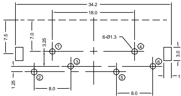
Recommended PCB Layout (Bottom View)
