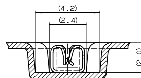
SECT. B-B
