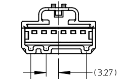
OPTION "A" OPTION "B" OPTION "C" VIEWED FROM MATE SIDE
