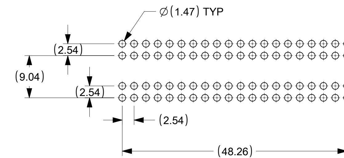
PCB LAYOUT FOR REFERENCE ONLY
