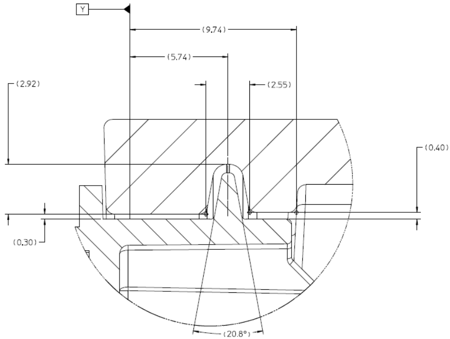
TYPICAL CONSTRUCTION DETAIL 7
