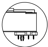
96/96 OR 96/72 MCMC HEADER WITH PCB SNAP LOCKING
