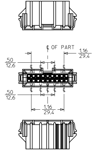
18 CIRCUIT
