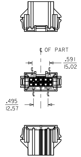
10 CIRCUIT
