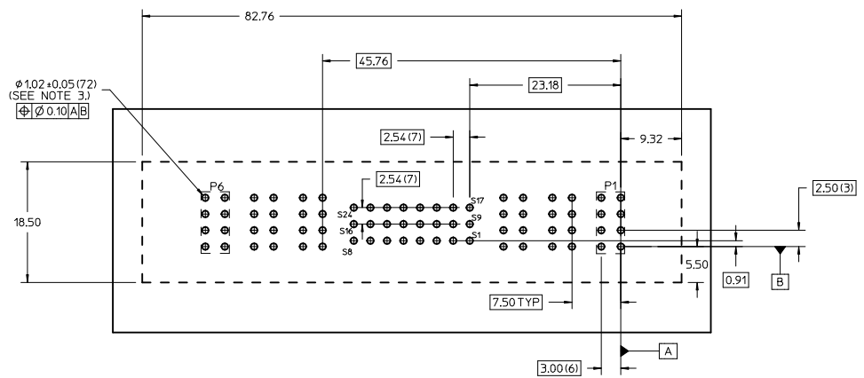
RECOMMENDED PCB LAYOUT AND KEEP-OUT ZONE
