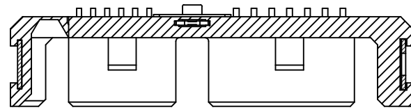
SECTION Z-Z
