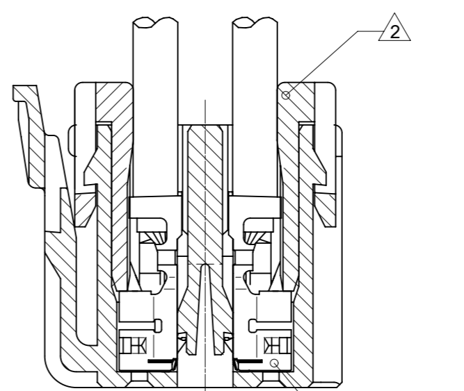
TERMINAL & RETAINER ASSEMBLY DRAWING SCALE 5:1
