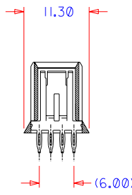
SECTION: Y-Y
