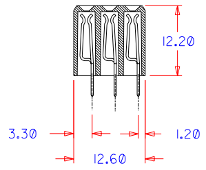
SECTION: Z-Z ROTATED 90° CW
