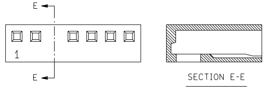
STD. VOID OPTION (VOIDS NOT AVAILABLE IN FIRST OR LAST CKT.)
