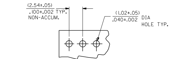
PCB LAYOUT: COMPONENT SIDE TYPICAL PCB THICKNESS: (1.57)/.062
