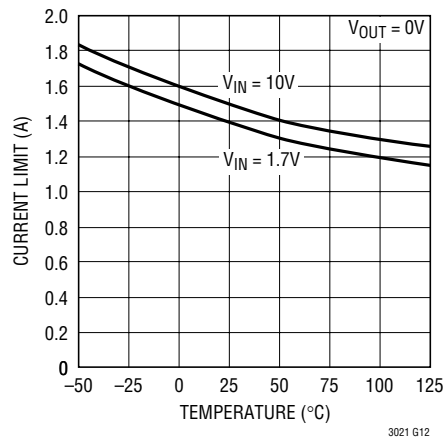
Current Limit
